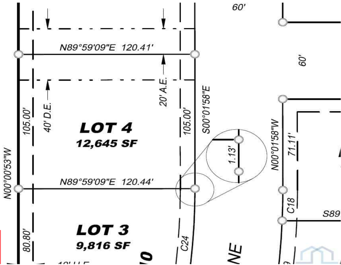
Lot 4 Block 10 Country Club Estates Elk Point City, Union County, SD
